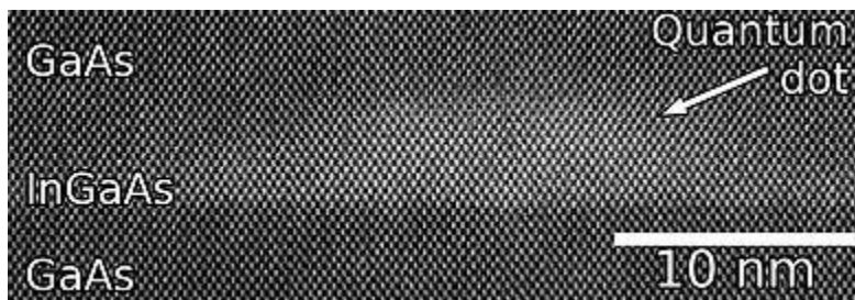
Atomic resolution scanning transmission electron microscopy image of an InGaAs quantum dot buried in GaAs.
